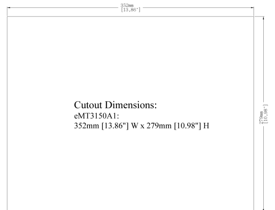
Panel Cutout
